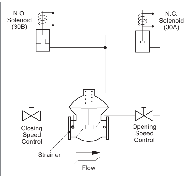
Figure 1. Model 210 Valve Schematic
